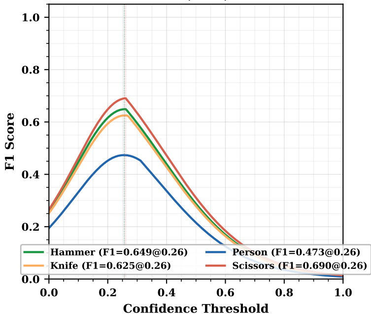
F1-Confidence Threshold Fine-tuned v5 (Final) — Test Set
